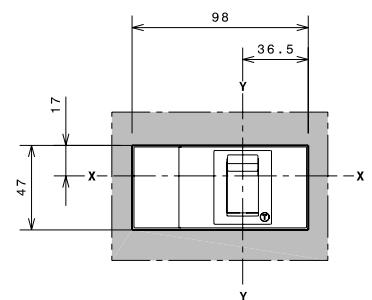
A = 61mm 4 poles
