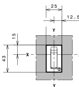
A = 69mm 1-2 poles
