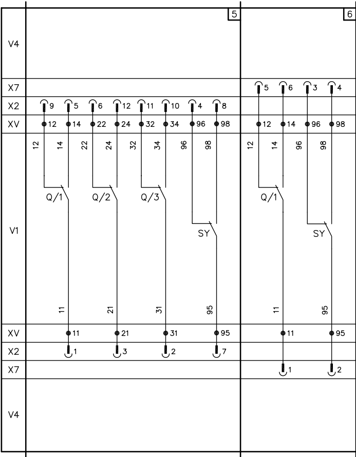
Figure: 5) Three changeover contacts for electrical signalling of circuit-breaker open/closed and one changeover contact for signalling circuit-breaker in tripped position due to thermal-magnetic trip unit, or SOR-C, or UVR-C intervention (3Q + 1SY) 6) One changeover contact for electrical signalling of circuit-breaker open/closed and one changeover contact for signalling circuit-breaker in tripped position due to thermal-magnetic trip unit, or SOR-C, or UVR-C intervention (1Q + 1SY)
