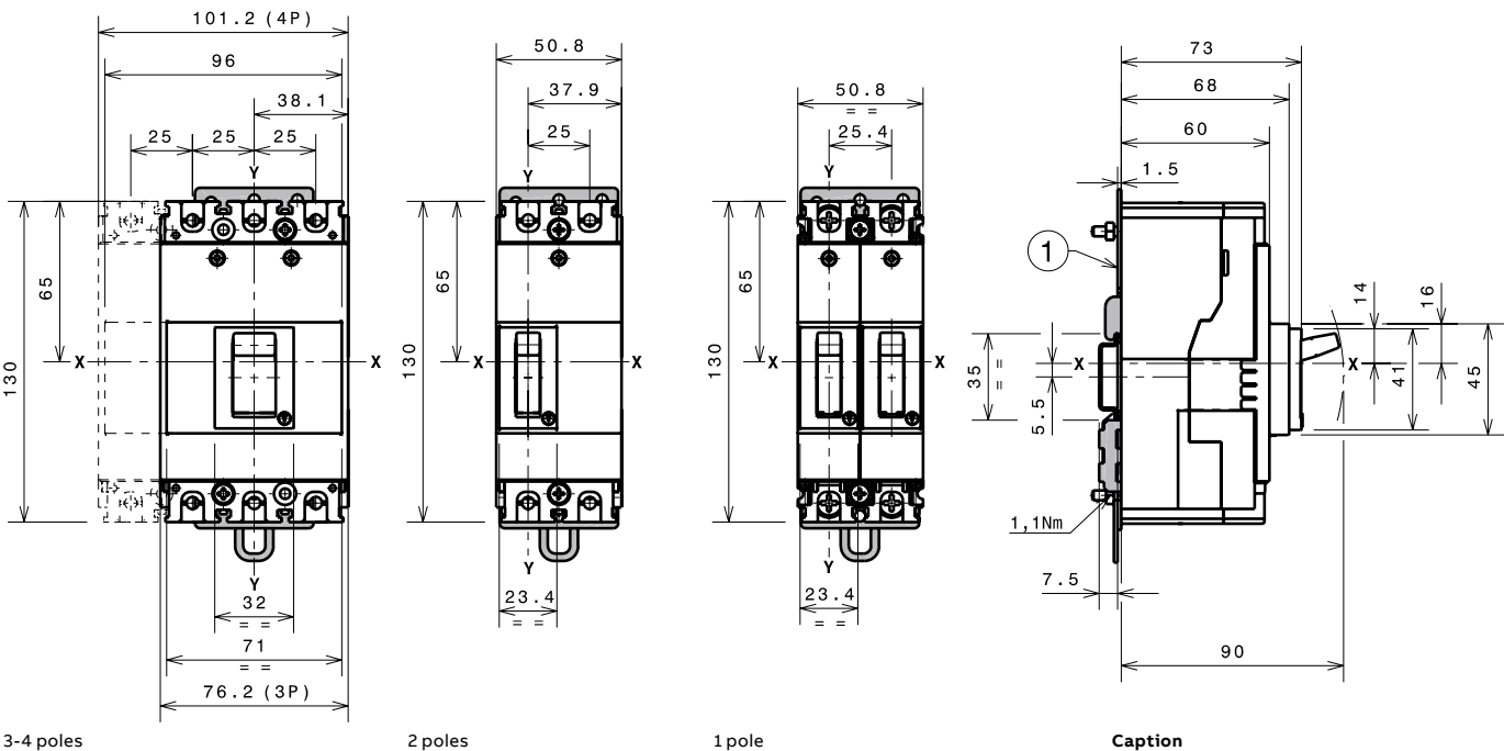
Caption ① Mounting bracket
