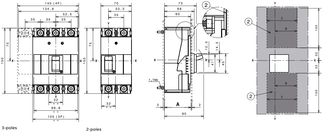
Caption ② Compulsory internal insulation plates (on customer's behalf) for use Ue ≥415 V
